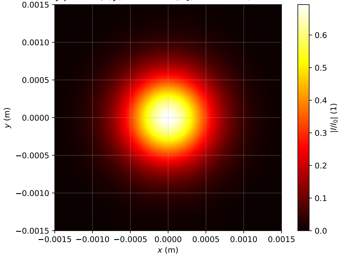
Intensity profile I(x, y, z = 2.468m)/I_0 , P_{in}=0.5P_{cr} , artificial time
